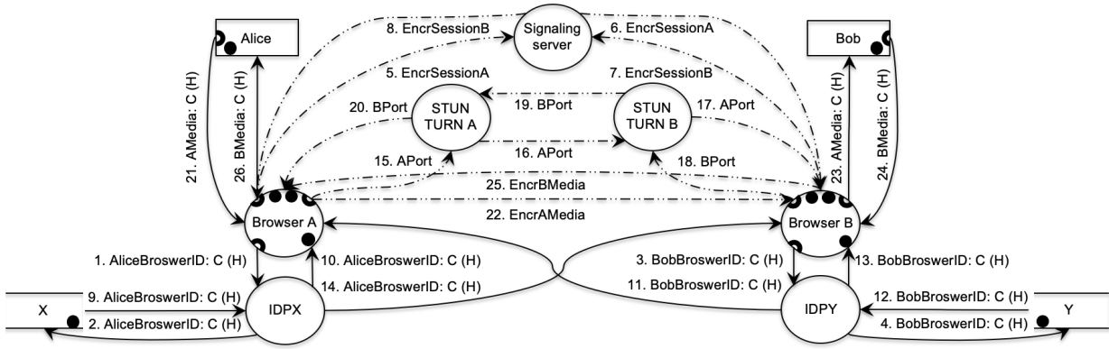
Fig. 8. A SecDFD for WebRTC after the analysis.
