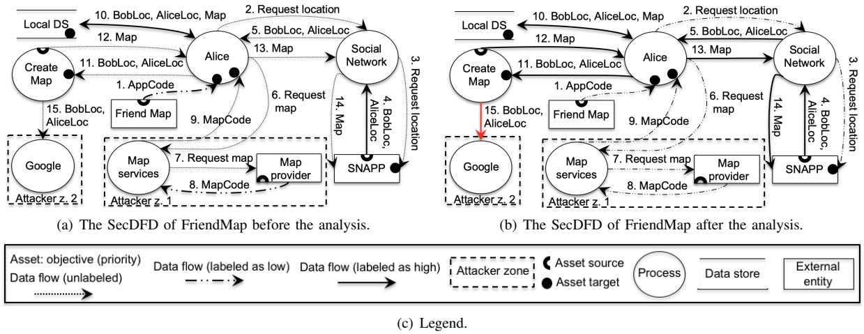
Fig. 1. A SecDFD of FriendMap before the analysis (a), after the analysis (b), and legend (c).
